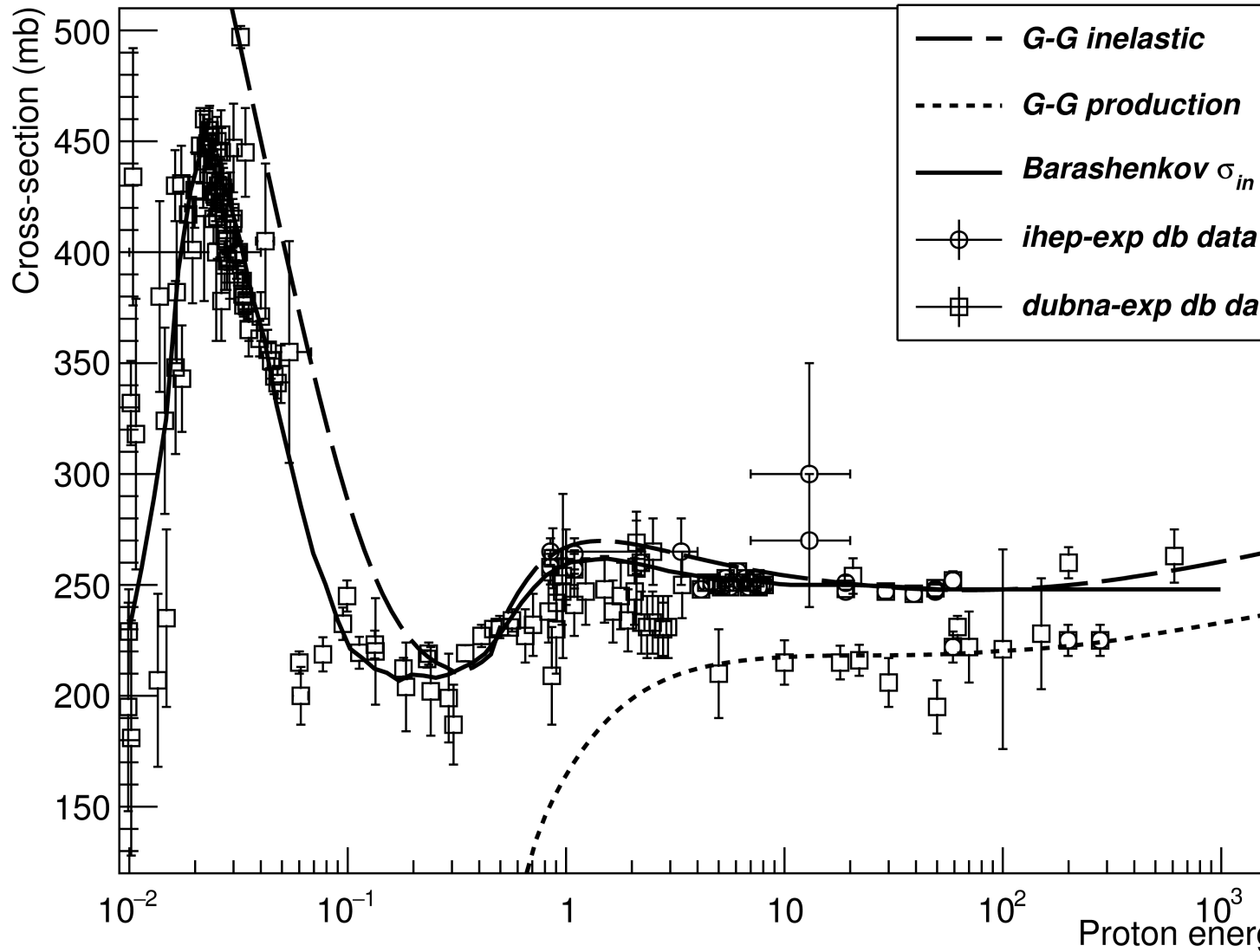
Fig. 21.2: Inelastic and production cross-sections of protons on a carbon target in the energy range 10^{-2} - 10^3 GeV. Experimental data (open points and squares) are from [IHEP][NEA]. The solid and dashed lines correspond to the Barashenkov and Glauber-Gribov inelastic models, respectively. The dotted line shows the Glauber-Gribov production model.
