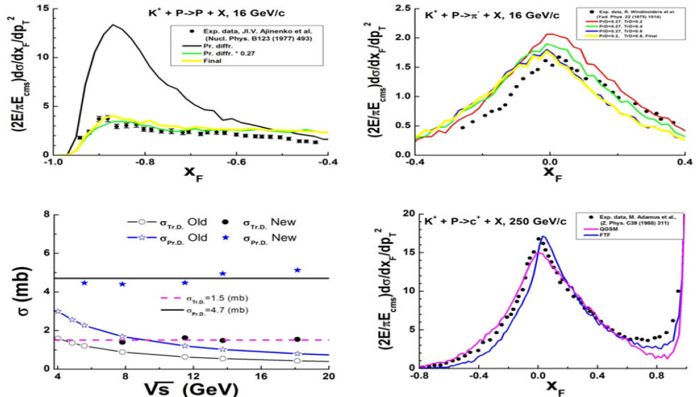
Fig. 25.13: Upper figures: inclusive spectra of protons and \pi^- -mesons in (Kp) -interactions. Points are experimental data [eal86][eal77]. Lines are FTF calculations. Bottom left figure: diffraction dissociation cross sections obtained by tuning (points), and their description (lines) by the expression for Kp in (25.4). Bottom right figure: x_F spectrum of positive charged particles in Kp -interactions at p_{lab} = 250 GeV/c. Points are experimental data [Whi74], lines are model calculations.
