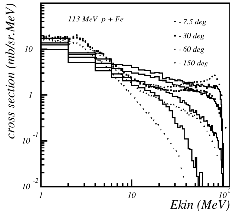
Fig. 27.5: Double differential cross-section for neutrons produced in proton scattering off Iron. Proton incident energy was 113 MeV. The points are data, the histogram is Binary Cascade prediction.
