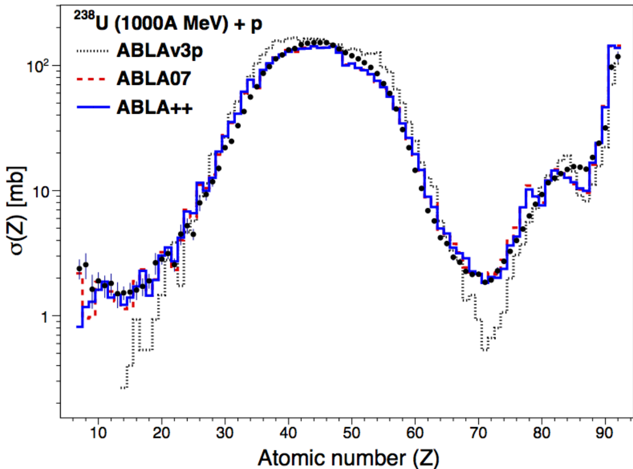
Fig. 34.1: ABLA calculations performed with the fortran version (ABLA07), the new one in C++ (ABLA++) and the previous version (ABLA v3p ) are compared with the atomic-number distribution of fission and evaporation residues produced in the reactions p + {}^{238}\text{U} at 1A GeV.
