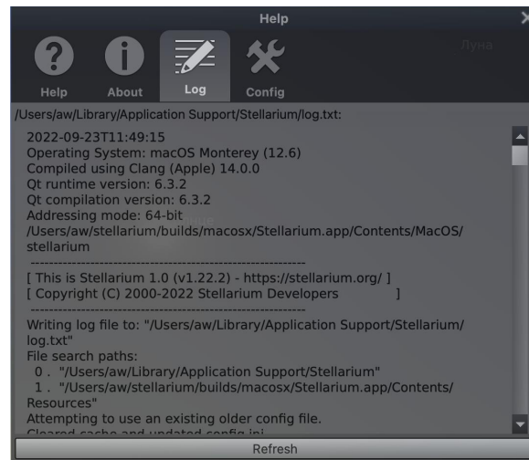
Figure 4.48: Help Window: Logfile
