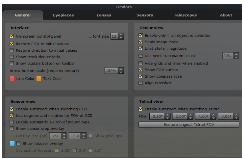
Figure 16.11: General tab of the Oculars plugin configuration dialog.
